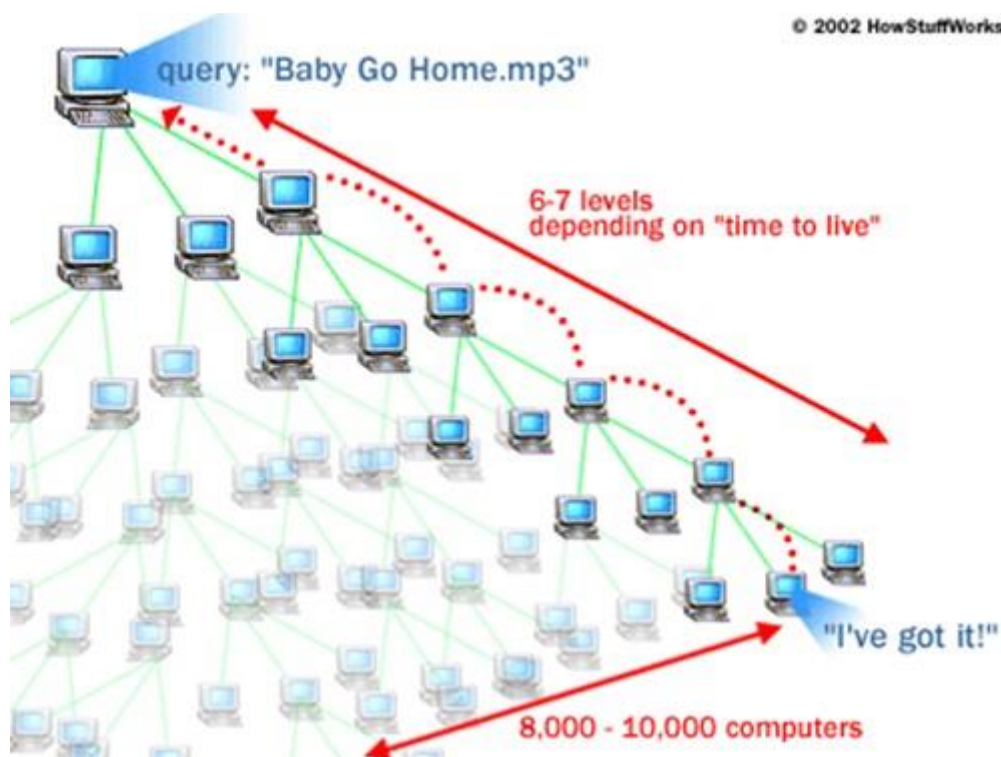
Figure 117: Grokster schematic
